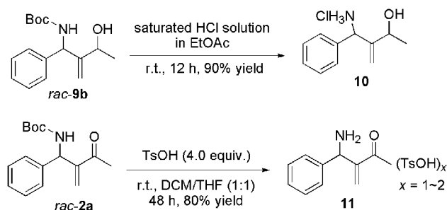
Scheme 6. Removal of the Boc group from adduct rac -2a or 9b .
