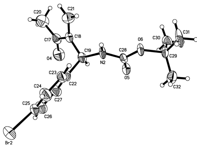
Figure 1. ORTEP drawing of compound 2d . [13]
