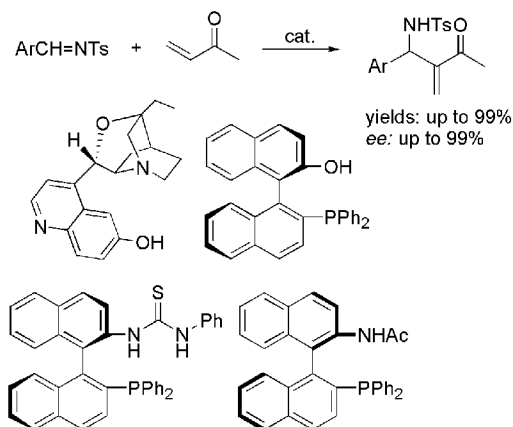
Scheme 1. Asymmetric aza-Morita-Baylis-Hillman reactions of N -sulfonated imines with MVK in our previous reports.
