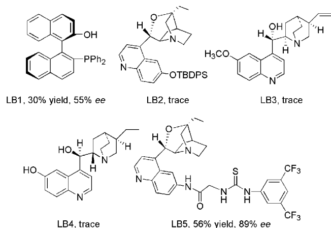
Scheme 2. Some chiral catalysts examined in the aza-MBH reaction of N -Boc imine 1a and MVK.
