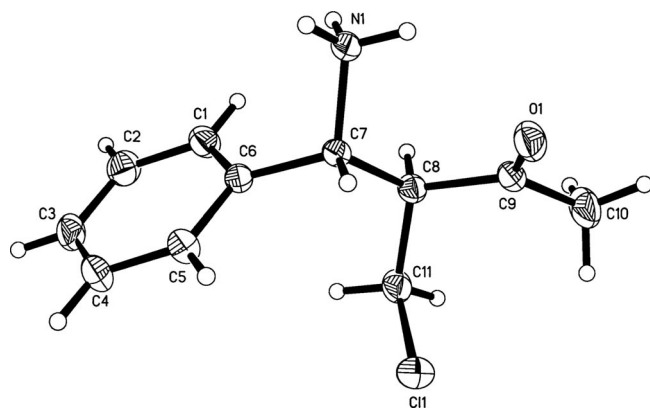
Figure 2. ORTEP drawing of compound 8a . [15]
