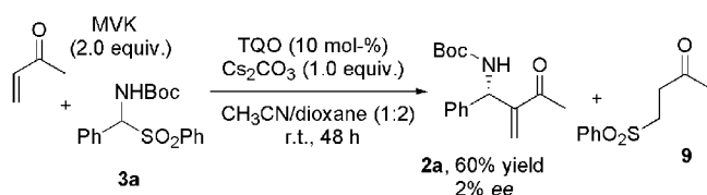
Scheme 3. The reaction of N -Boc α-amidoalkyl phenyl sulfone 3a with MVK in the presence of cesium carbonate by using TQO as the catalyst.
