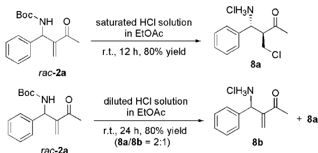
Scheme 5. Removal of the Boc protecting group from adduct rac -2a.
